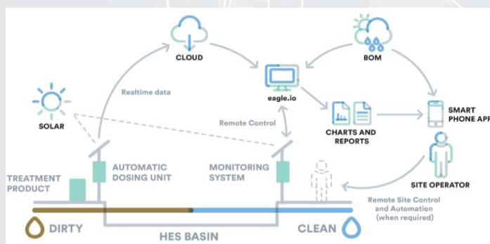
Figure 2 – High Efficiency Sediment Basin Flowchart
